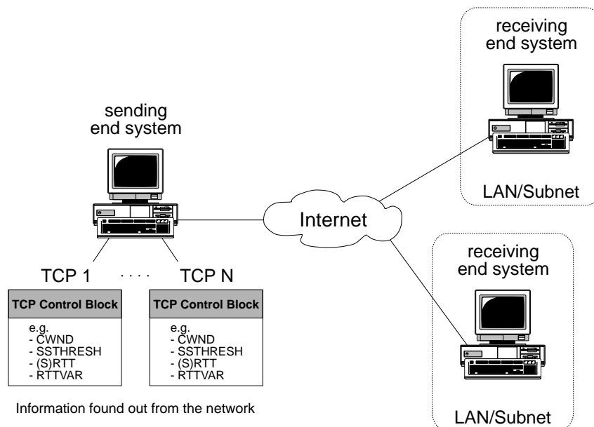
Fig. 1. The TCP control blocks of N TCP senders of an end system
