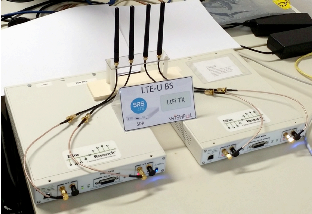
Figure 1. Two USRP X310 used to test LTE-MIMO.
