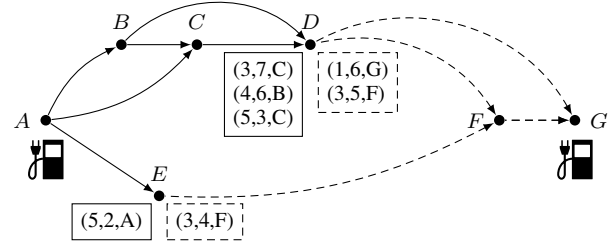
(b) Forward and backward shortest-path trees with labels of common nodes. Solid: Forward tree from node A. Dashed: Backward tree from node G
