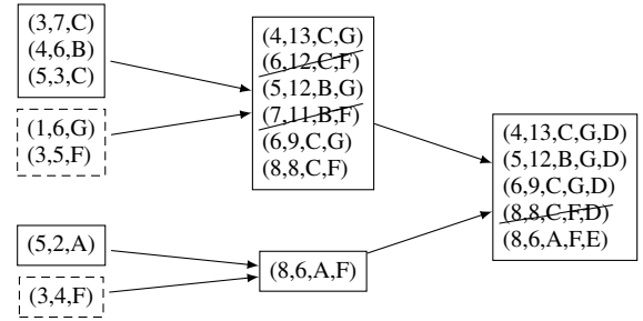
(c) Create sumsets from node labels and combining them to get resulting Pareto set
