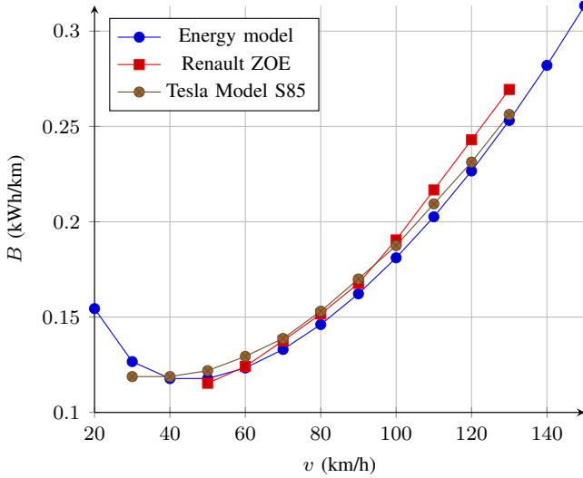
Figure 5. Energy model compared to energy consumption of two real electric vehicles
