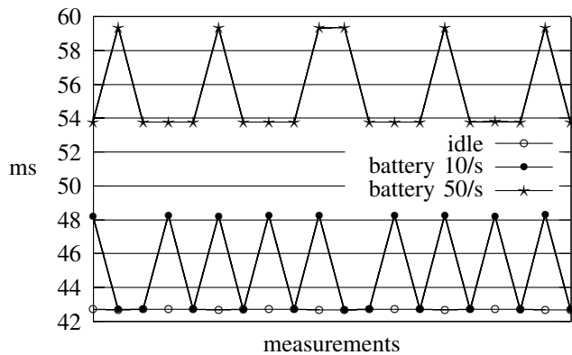
Fig. 8. Hashing 1024 byte of data with MD5 while measuring the battery voltage
