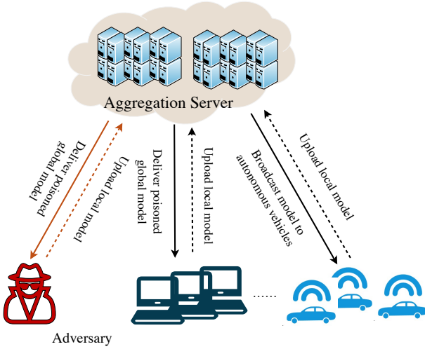
Fig. 11. Workflow of an FL poisoning attack presented in [121]. The adversary manipulates the local training process to upload poisoned models. The aggregation server fails to detect the malicious updates and integrates them into the global model, which is then disseminated to all connected devices, compromising system integrity.
