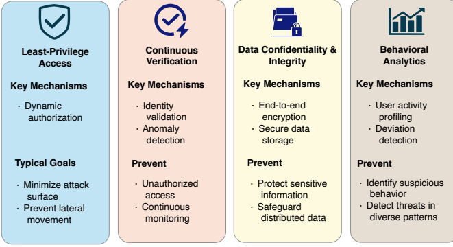
Fig. 6. Core principles of ZTFM in IoT environments. Each principle – LPA, continuous verification, data confidentiality & integrity, and behavioral analytics – maps to specific mechanisms and goals designed to enhance security posture in distributed, heterogeneous IoT systems.
