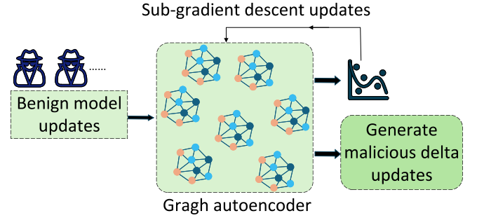
Fig. 3. An illustration of an adversarial variational graph autoencoder-enabled model poisoning attack [64].
