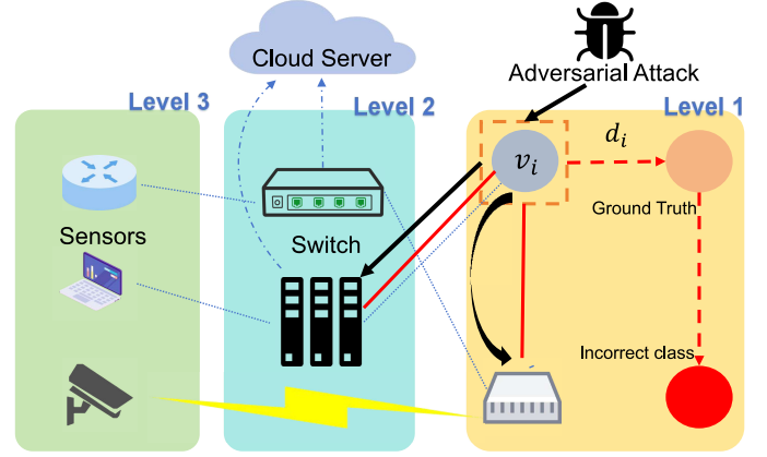
Fig. 4. An illustration of hierarchical black-box adversarial attacks on GNN-based NIDS in IoT networks [84]. Here, adversaries exploit multi-level infrastructure and graph feature perturbations to induce misclassifications while bypassing intrusion detection systems.
