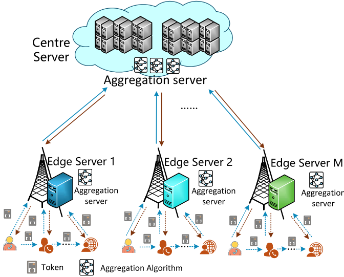
Fig. 7. A representative architecture of privacy-preserving FL in edge computing [110]. This hierarchical structure incorporates local aggregation at edge servers and global coordination by a central server, supporting secure multiparty computation and token-based update verification among distributed IoT users.
