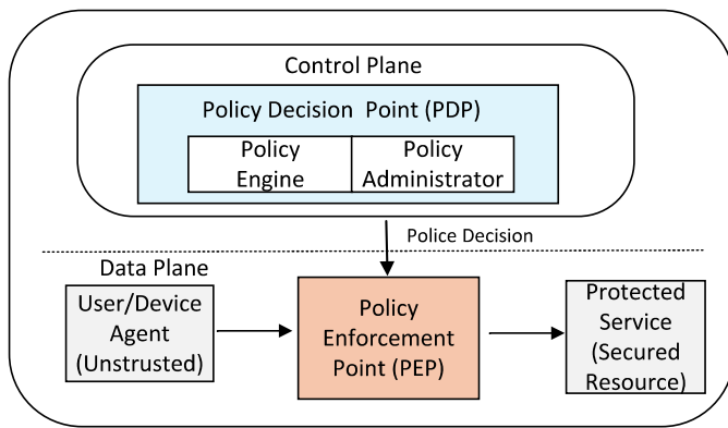
Fig. 9. The core structure of the zero-trust architecture proposed in [114], which delineates the control plane, where the Policy Decision Point (PDP) governs access logic, from the data plane, where the Policy Enforcement Point (PEP) mediates all subject–resource interactions. The separation ensures scalable, policy-driven trust enforcement across dynamic environments.
