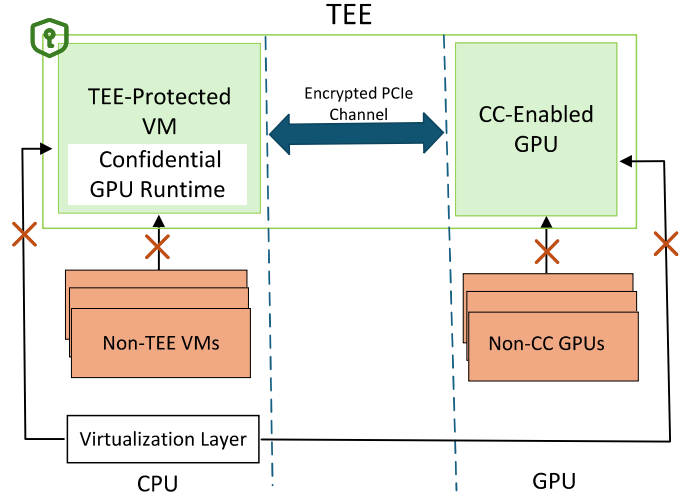
Fig. 8. An illustration of a CPU-GPU co-architecture for confidential computing using a TEE, as developed in [111]. Encrypted PCIe channels and enclave-based isolation prevent unauthorized access from legacy VMs or GPUs, highlighting the role of secure virtualization and hardware-assisted attestation in zero-trust computing environments.
