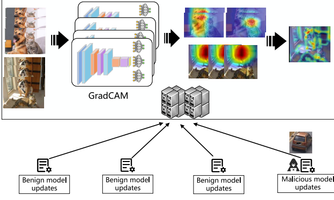
Fig. 5. An illustration of the GradCAM-based defense mechanism against model poisoning attacks developed in FMs [89].
