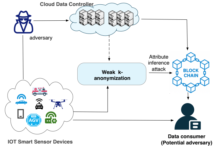
Fig. 10. Overview of a potential privacy breach in blockchain-based IoT data sharing [121]. This attacker model illustrates the end-to-end flow of data from IoT devices to adversarial consumers, emphasizing the risks of using weak anonymization and highlighting the need for stronger privacy-preserving mechanisms in Zero-Trust IoT ecosystems.
