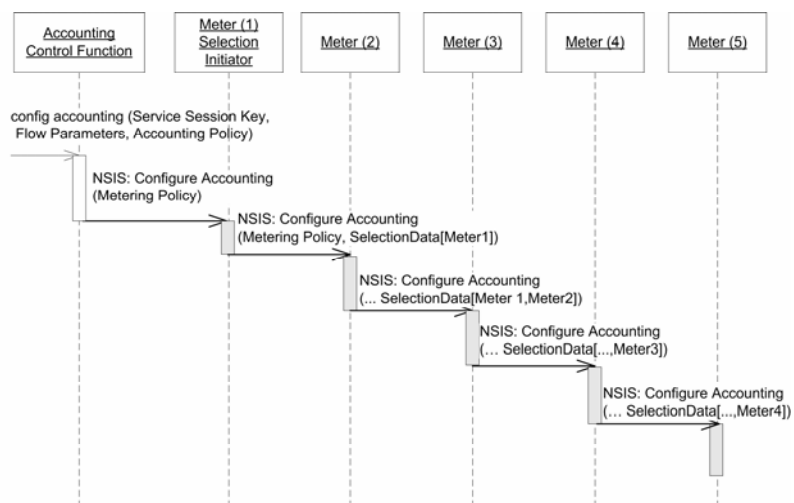
Figure 3: Meter Selection Message Exchange
