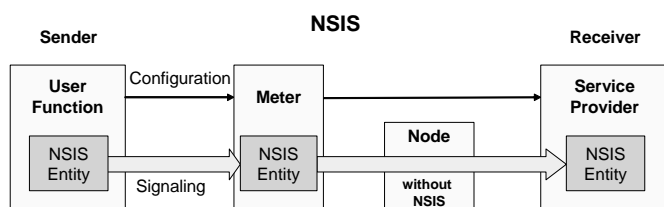
Figure 2: NSIS Signalling
