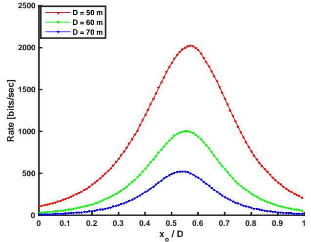
FIGURE 9. Achieved Rate versus \frac{x_o}{D} for different at D = 50, 60 and 70 m.
