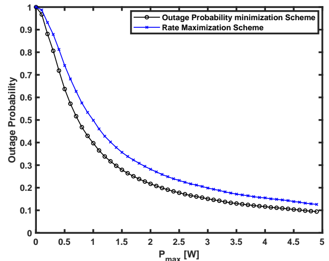
FIGURE 10. Achieved Outage Probability versus P_{max} when using Optimum Powers for Outage Probability Minimization Algorithm and Optimum Powers for the Rate Maximization Algorithm, respectively.
