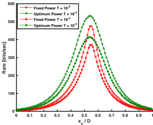
FIGURE 8. Achieved Rate versus \frac{x_o}{D} for different T values at D = 70 m.
