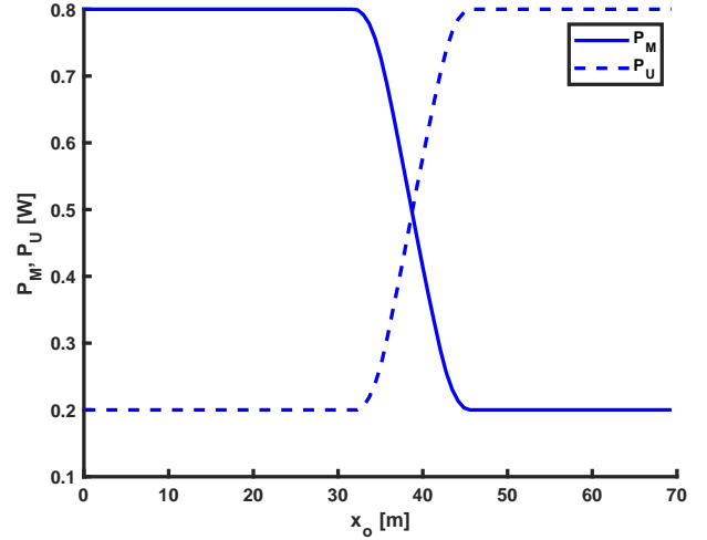
FIGURE 6. P_M and P_U at different locations of the UAV at D = 70 m.
