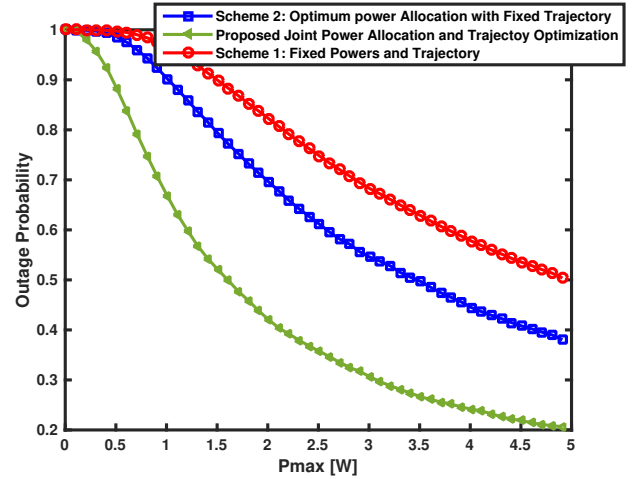
FIGURE 3. Outage Probability achieved through the fixed power and trajectory, optimum power allocation with fixed trajectory and joint power allocation and trajectory optimization schemes vs. P_{max} for x_o = 60 m, y_o = 0 , z_o = 22.5 m.
