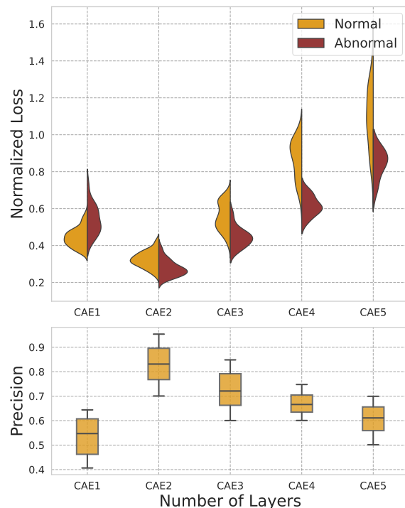
Fig. 6: Reconstruction error distribution for SS-DeepCAE with different layer size (Upper Graph) Precision distribution of SS-DeepCAE with different layer size (Lower Graph)
