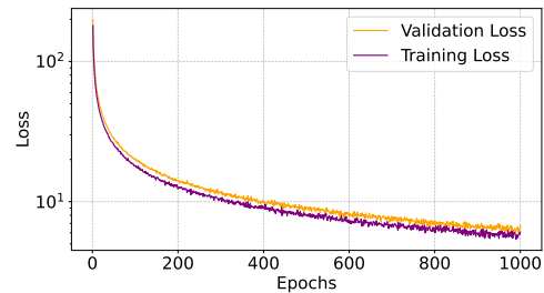
(a) Training/Validation Loss.
