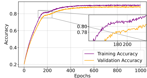
(b) Training/Validation Accuracy.
