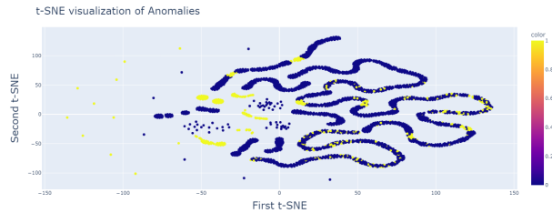
Fig. 4: Dimensionality reduction on our high-dimensional unbalanced data (yellow color represent anomalous samples, blue color represents non-anomalous samples)
