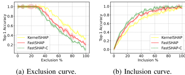
Fig. 9: Exclusion and Inclusion Curves for top-1 Accuracy
