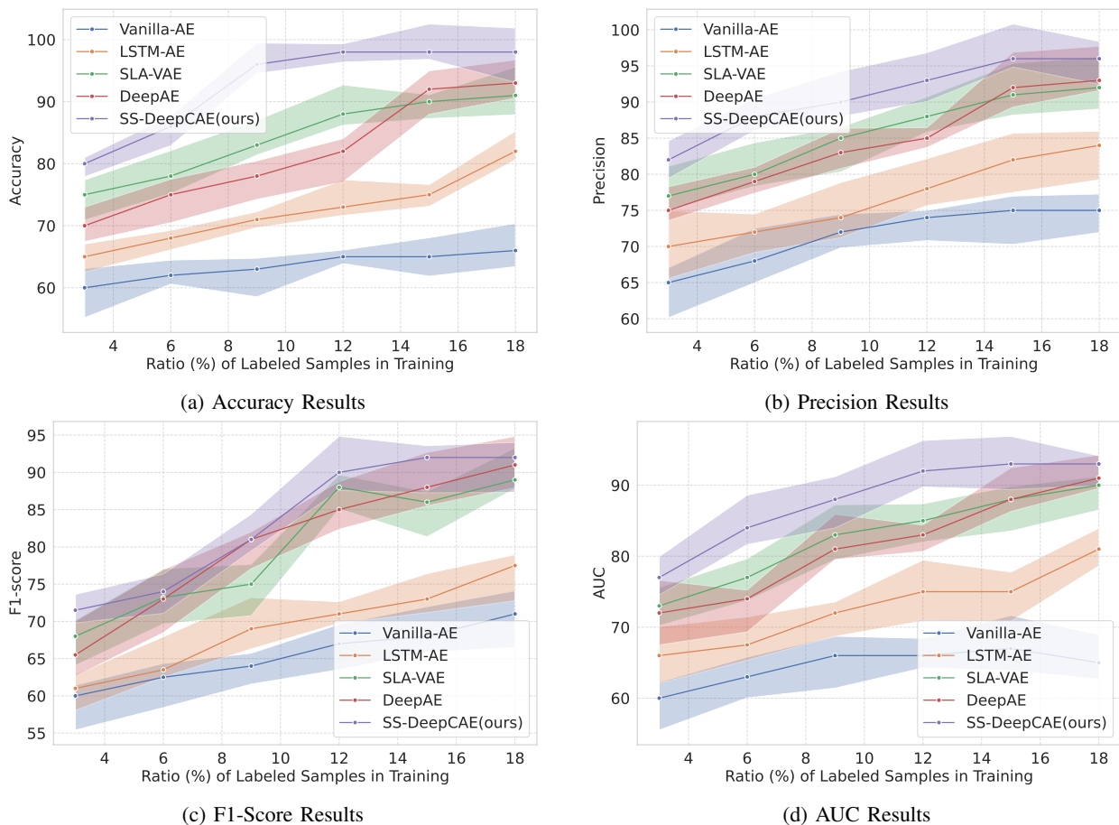
Fig. 7: Accuracy, Precision, F1-score, and AUC variation curves of models with different ratio labeled samples
