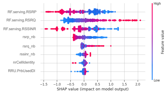
Fig. 8: Explaining feature contributions with SHAP values
