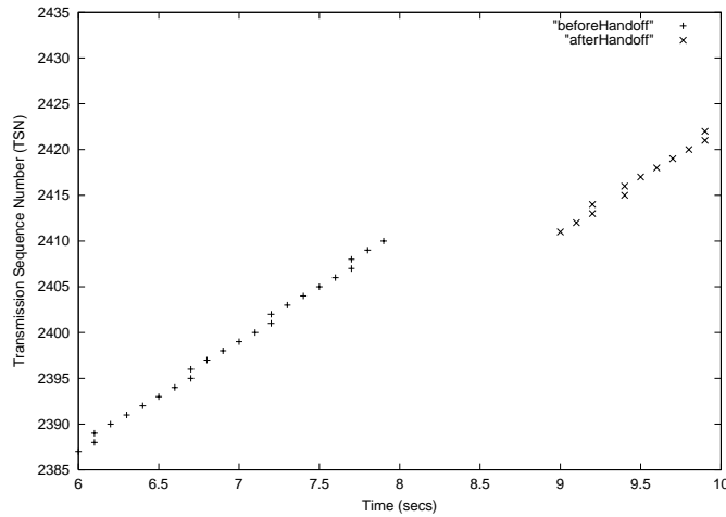
Figure 4. An SCTP association sequence trace during handoff
