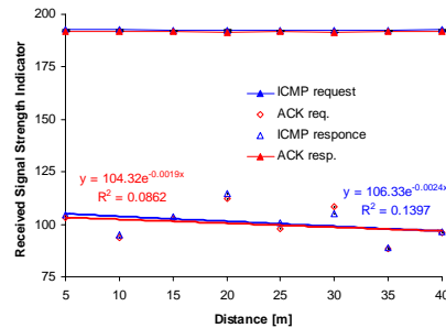
Fig. 4. Distance as calculated from RTT Fig. 5. Received signal strength indicator versus actual distance between both nodes. 95% confidence levels are given.
